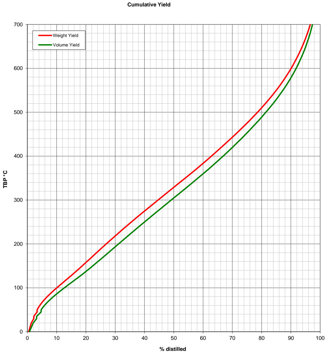
Cumulative Volume % Distilled at 10 Degree C (TBP) Intervals
